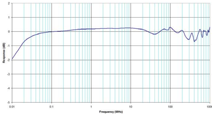
Model HI-6122 Typical Frequency Response
